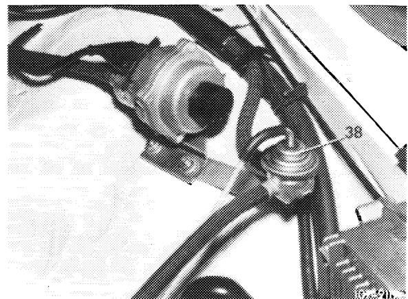
Layout model year 1974 38 Purge valve (draw-off valve)
