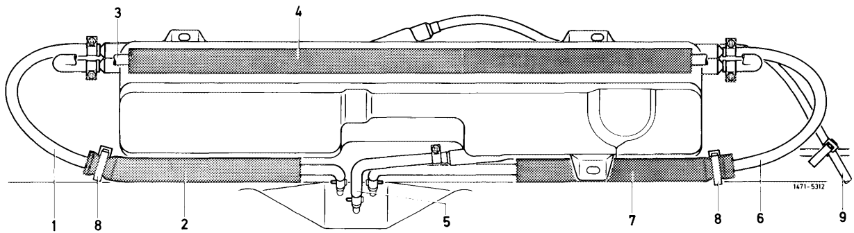
Fuel expansion tank with 5 connections
