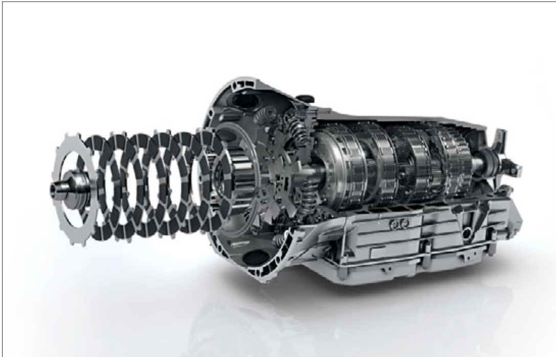
Fast and easy: changing gear with the AMG SPEEDSHIFT MCT 7-speed sports transmission
