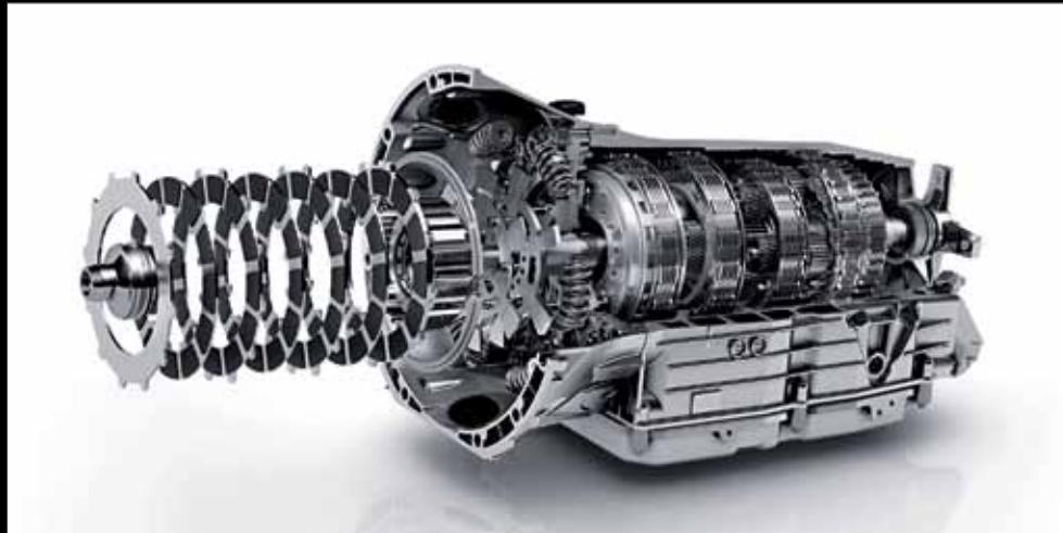
5-speed automatic transmission with AMG SPEEDSHIFT enhancements.
