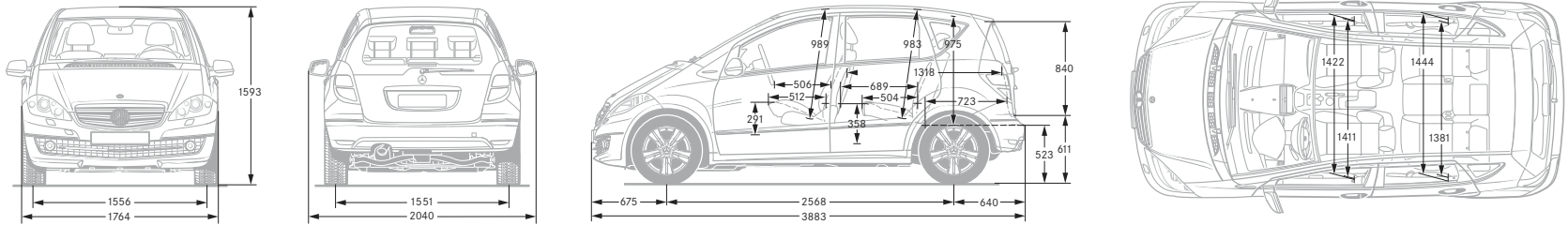
Figures in brackets apply to the A 160 CDI Coupé with manual transmission and sports suspension. All measurements in millimetres. The dimensions shown are mean values and apply to standard-specification, unladen vehicles
